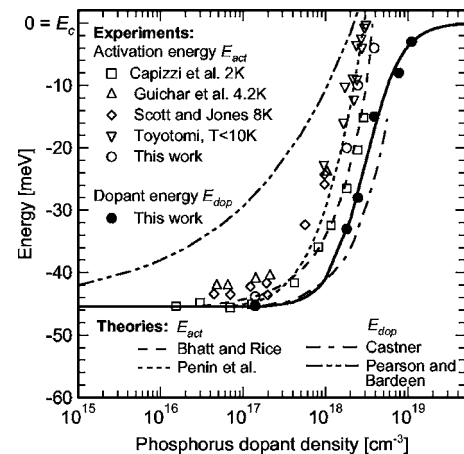
FIG. 3. The energy of the dopant band peak E_{\text{dop}} (filled circles) and the activation energy of the dopant band E_{\text{act}} (empty circles), as derived from Fig. 1. The other symbols show E_{\text{act}} values, obtained from various measurement techniques (Refs. 36, 37, 39, and 125). The solid line is the parametrization using Eq. (7). The dashed lines show theoretical computations (Refs. 5, 42, 99, and 107).
